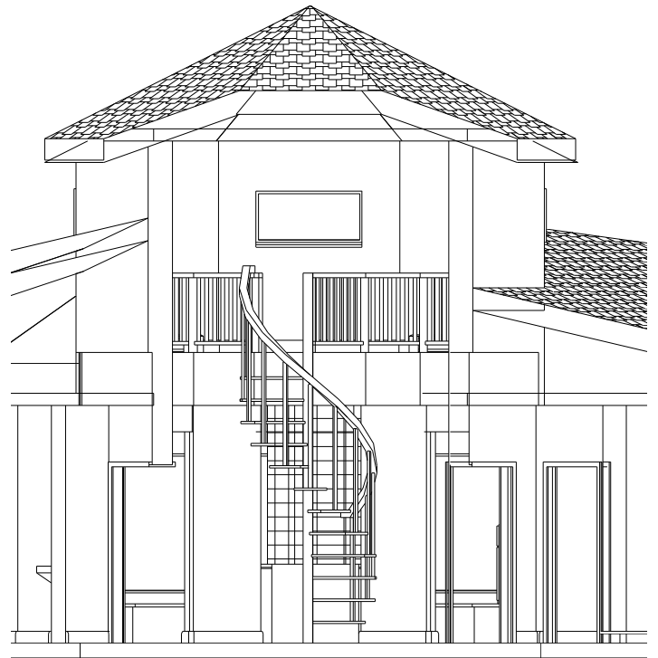
Tower elevation from rear
